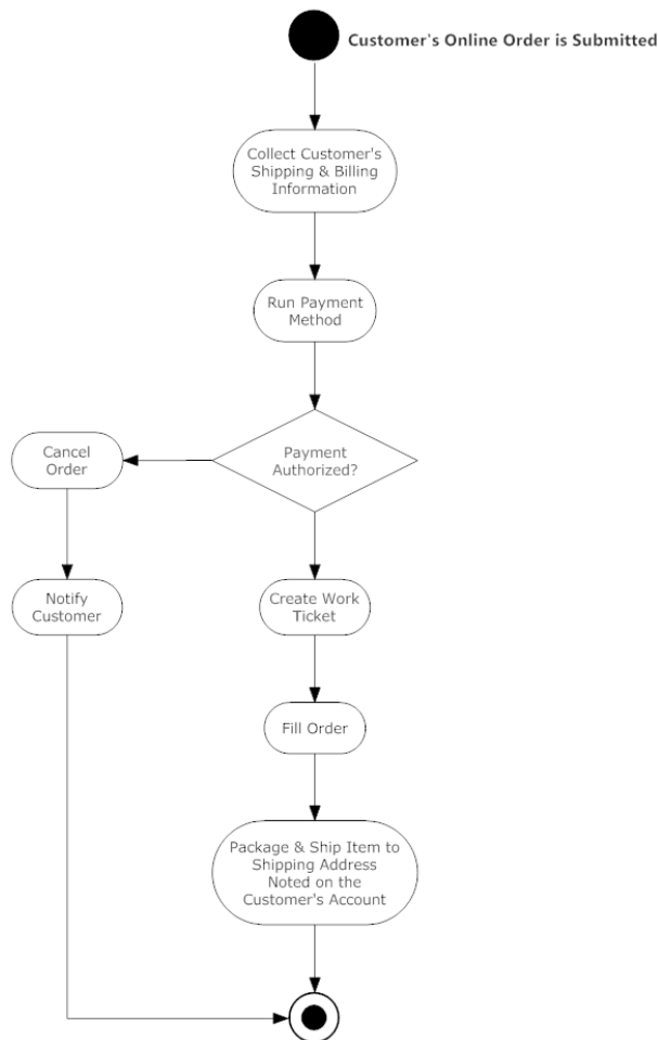
Online Order Activity Diagram
